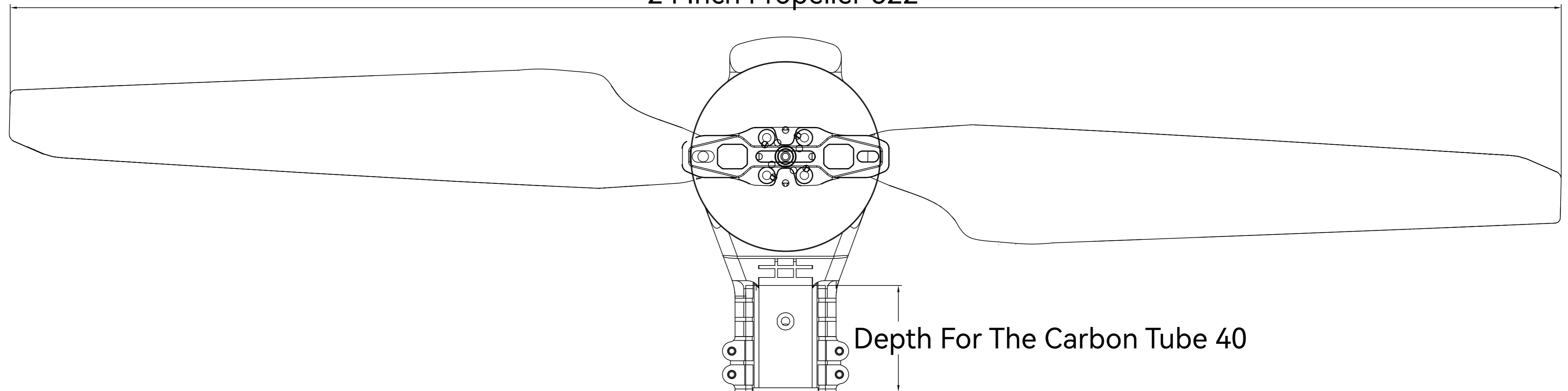
24 Inch Propeller 622
