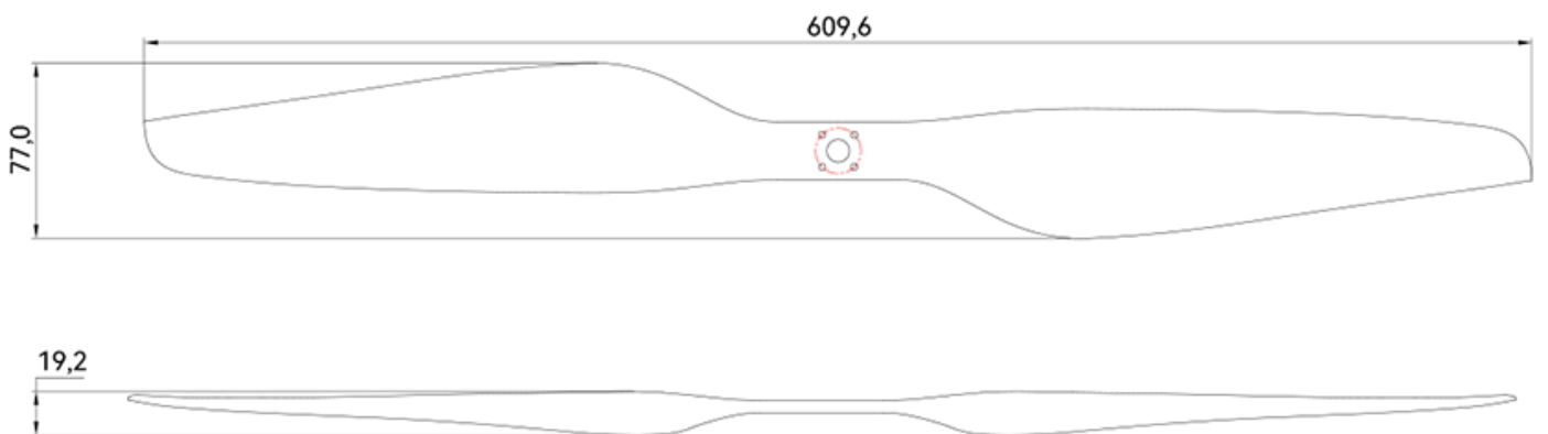
[PROPELLER]
