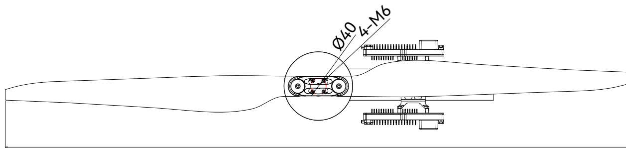
63 Inch Propeller 1600.20
